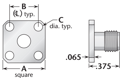
Figure 1 (1/2" square flange)
