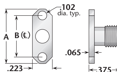
Figure 2 (2-hole flange)
