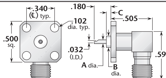
Figure 1 (Solder pot contact)
