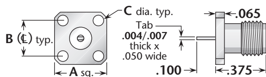
Figure 1 (3/8" square flange)
