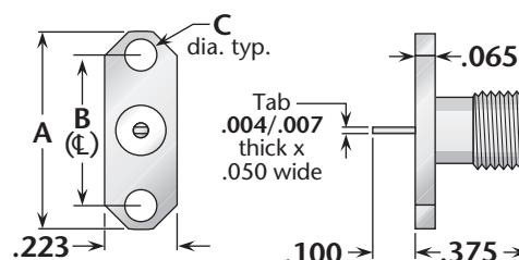
Figure 5 (2-hole flange)
