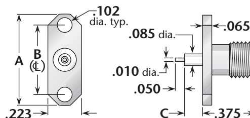
Figure 5 (2-hole flange)
