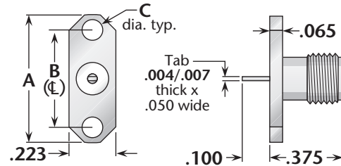
Figure 5 (2-hole flange)
