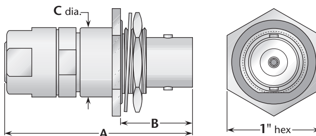
Figure 1 (Rear mount)
