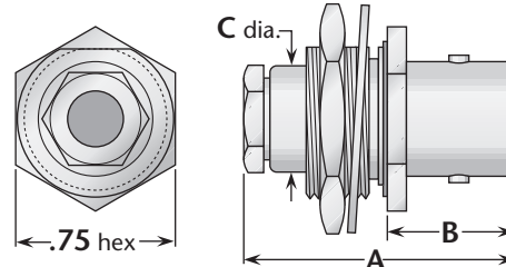
Figure 2 (Front mount)
