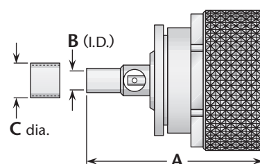
Figure 3 (Solder type for semi-rigid cable)
