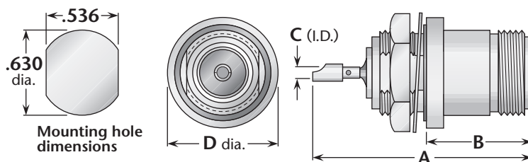
Figure 1 (Bulkhead jack, hermetically sealed)
