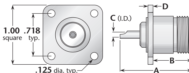
Figure 2 (Panel jack)
