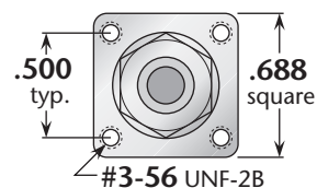
Flange dimensions
