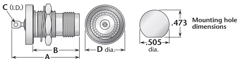
Figure 1 (Rear mount)
