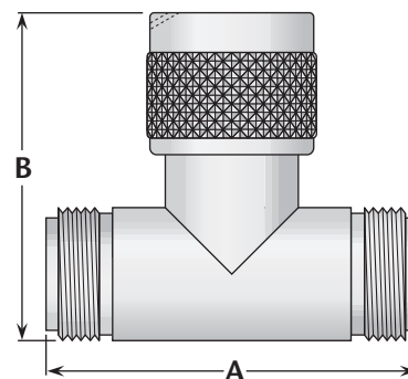
Figure 4 (Tee, jack-plug-jack)
