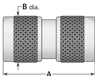
Figure 3 (Straight plug-plug)
