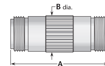
Figure 6 (Straight jack-jack)
