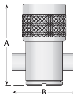
Figure 2 (Direct solder for semi-rigid cable)
