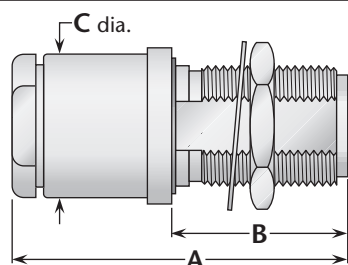
Figure 1 (Rear mount)
