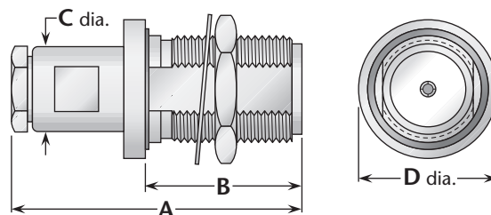
Figure 2 (Rear mount)
