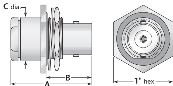
Figure 1 (Rear mount)
