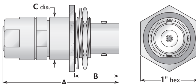
Figure 1 (Rear mount)
