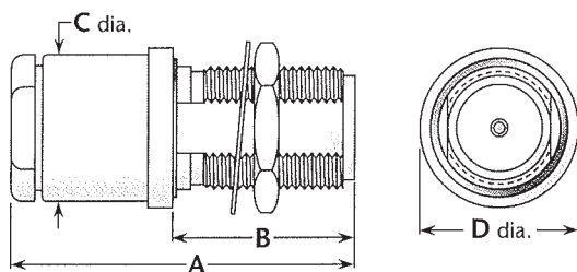
Figure 1 (Rear mount)
