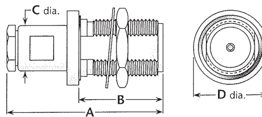
Figure 2 (Rear mount)
