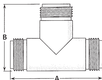
Figure 1 (Tee jack-jack-jack; connects three plugs)
