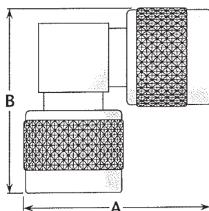
Figure 2 (Right angle plug-plug; connects two jacks)
