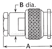
Figure 4 (Safety-wire holes in coupling nut)
