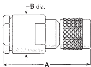
Figure 1 (Standard coupling nut)
