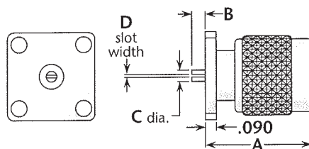
Figure 3 (Slotted contact, 11/16" square flange)
