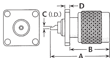
Figure 1 (Solder pot contact, 3/4" square flange)
