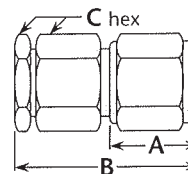
Figure 2 (Clamp type)
