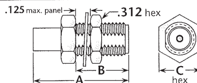
Figure 2 (Bulkhead mount, direct solder)
