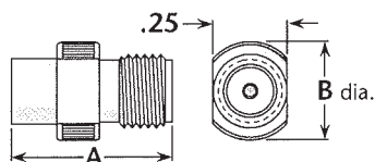
Figure 1 (Straight jack, direct solder)
