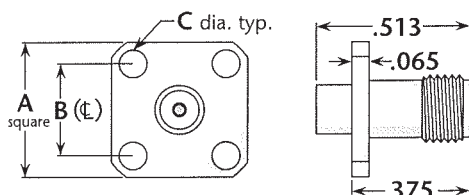
Figure 3 (4-hole flange, direct solder)
