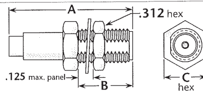
Figure 4 (Bulkhead jack)
