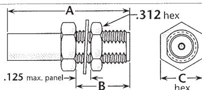
Figure 3 (Bulkhead jack)
