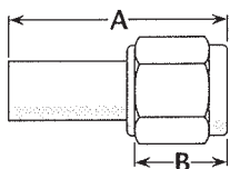
Figure 1 (Straight plug)
