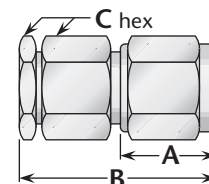
Figure 2 (Clamp type)
