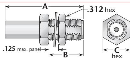
Figure 3 (Bulkhead jack)
