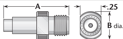
Figure 2 (Straight jack)
