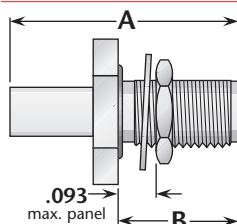
Figure 3 (Direct solder, with mounting gasket)
