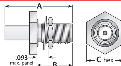
Figure 5 (One-Step cable attachment, with mounting gasket)
