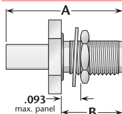
Figure 3 (Direct solder, with mounting gasket)
