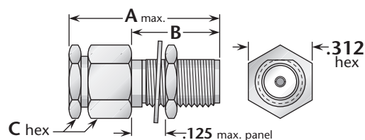
Figure 2 (Clamp type)
