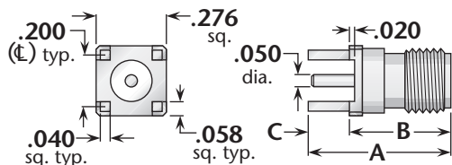
Figure 1 (Straight jack)
