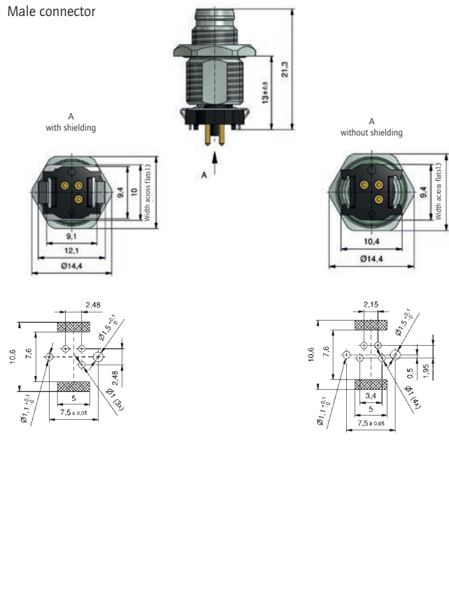
Male connector
