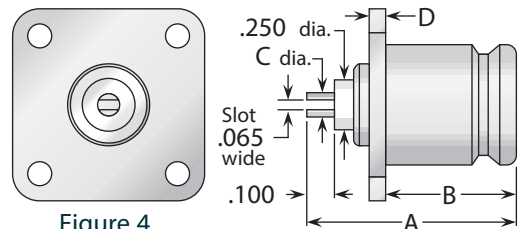
Figure 4 (Slotted contact)
