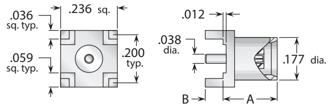
Figure 2 (Through-hole mount)
