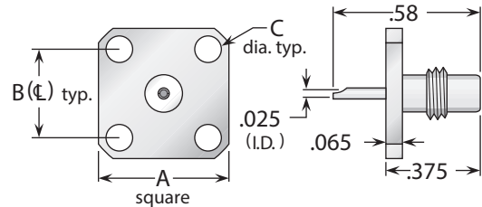
Figure 2 (1/2" square flange)
