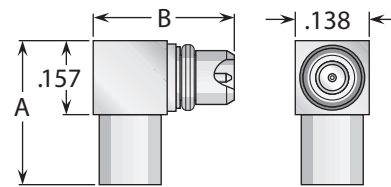
Figure 4 (Right angle direct solder for semi-rigid cable)
