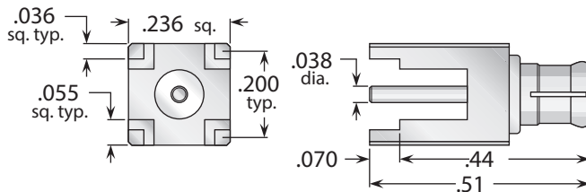
Figure 1 (Straight—through-hole mounting)
