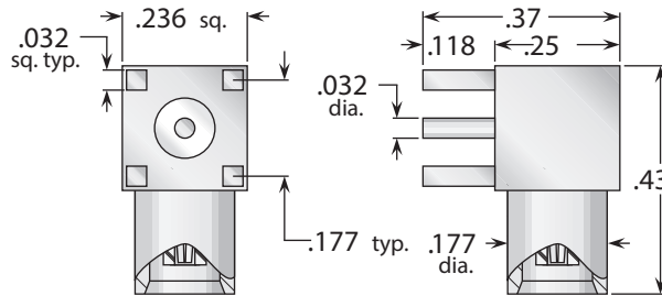
Figure 1 (Through-hole mount)
