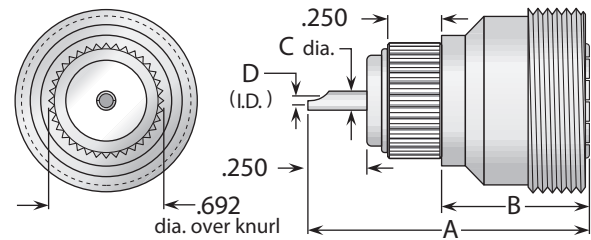
Figure 4 (PressMount)
