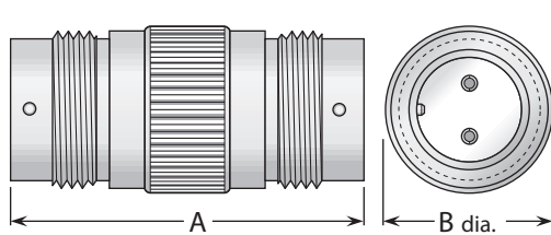
Figure 1 (Straight jack-jack; connects two plugs)
