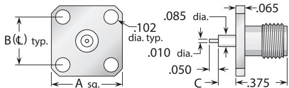
Figure 2 (1/2" square flange, SMA standard flange size)
