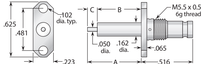
Figure 2 (2-hole flange)
