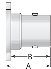
Figure 3 (Dummy receptacle)
