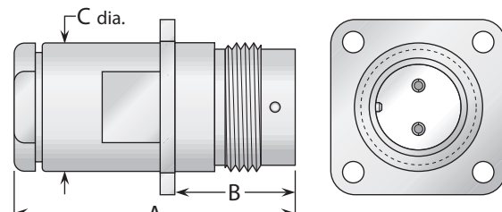
Figure 2 (Panel jack)
