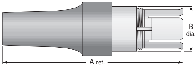
Figure 1 (Non-locking)
