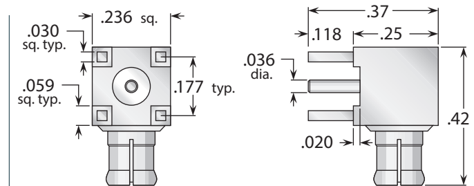
Figure 2 (Right angle—through-hole mounting)
