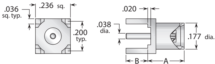
Figure 1 (Through-hole mount)
