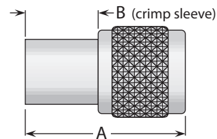
Figure 2 (Crimp type)
