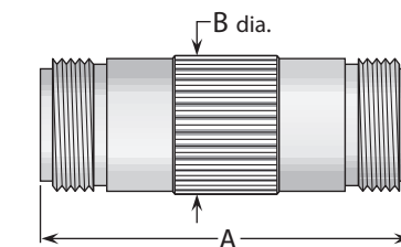
Figure 6 (Straight jack-jack)
