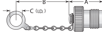
Figure 2 (Cap for TNC plug)
