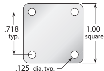
Flange Dimensions
