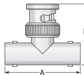
Figure 7 (Tee, jack-plug-jack)
