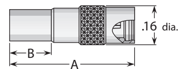
Figure 3 (Direct solder for semi-rigid cable)
