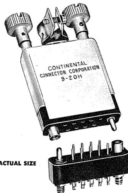
TYPE 144-6 hood and screwlock assembly
