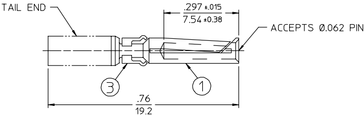
2 PIECE SOCKETS
