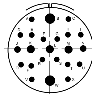
40-4 16-#16, 2-#12, 3-#8, 2-#4
