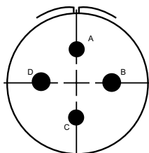
22-4 2-#12, 2-#8
