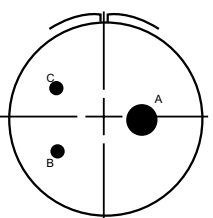
22-21 2-#16, 1-#0
