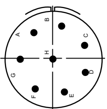
22-23 8-#12
