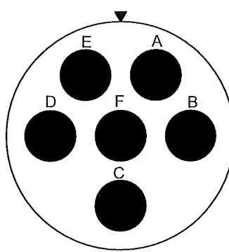
17-6/16-6 E6, 6 #12, I
