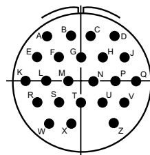
24-80 23-#16
