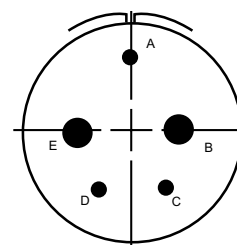
28-5 2-#16, 1-#12, 2-#4
