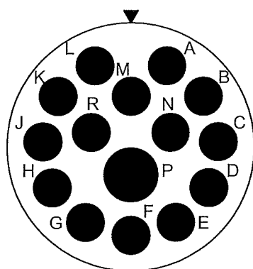
15-15/14-15 D15, 1 #16, 14 #20, I
