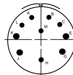
28-19 6-#16, 4-#12
