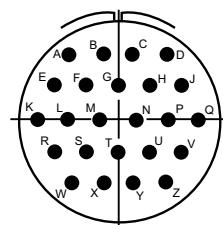
24-28 24-#16
