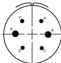
22-5 4-#16, 2-#12
