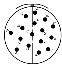
24-24 16-#16
