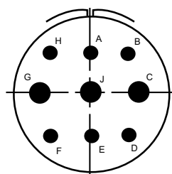
28-1 6-#12, 3-#8
