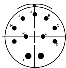
24-20 9-#16, 2-#12
