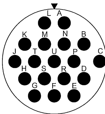
15-18/14-18 D18, 18 #20, I
