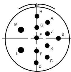
28-8 2-#12, 10-#16
