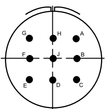
22-20 9-#16
