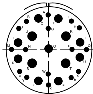
40-10 16-#16, 9-#8, 4-#4
