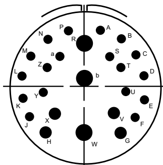
40-11 18-#16, 4-#12, 1-#8, 1-#4, 1-#0
