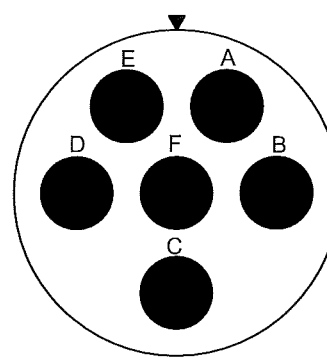
16-7 6 #12, II
