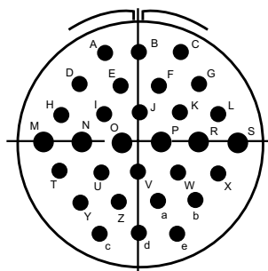
40-1 24-#16, 6-#12
