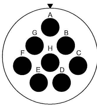
17-8/16-8 E8, 8 #16, II
