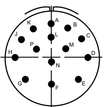
22-19 14-#16
