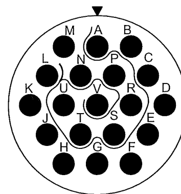
15-19 D19, 19 #20, I
