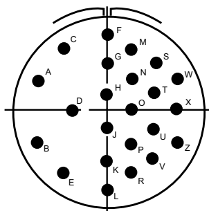
40-2 23-#16
