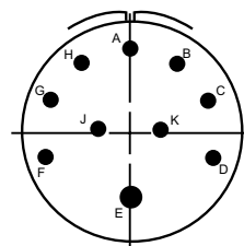
24-21 9-#16, 1-#8
