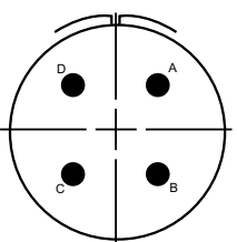
22-22 4-#8
