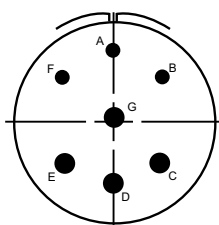
24-16 3-#16, 1-#8, 3-#12
