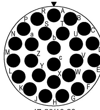
17-26/16-26 E26, 26 #20, I
