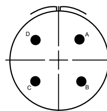
24-22 4-#8
