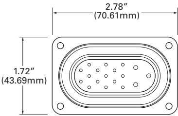
18 Pin Configurations
