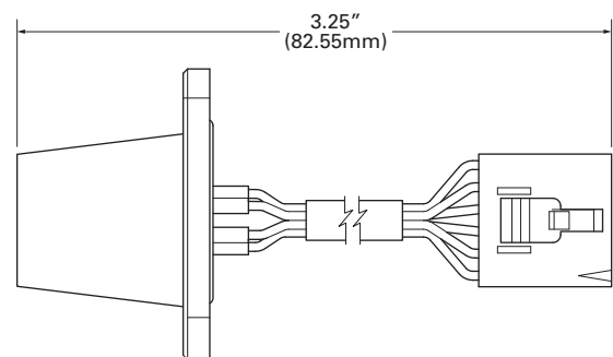
GCA3256628-1 cable assembly includes GCA3167930-3 connector
