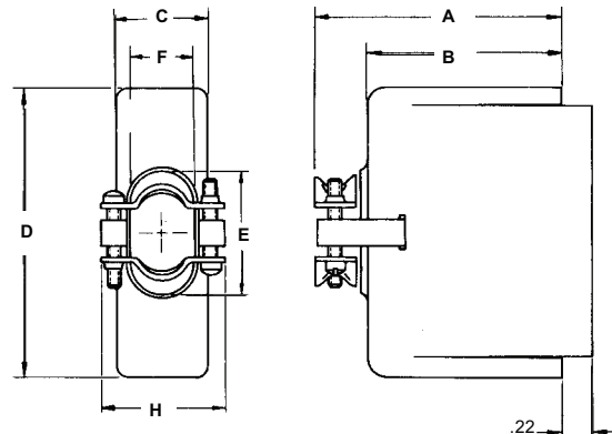
Style H8 / H13 — Top Cable Opening
