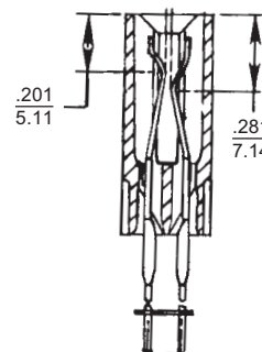
Early/Late Make Contacts
