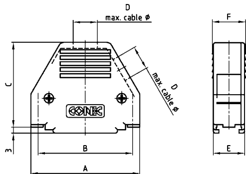
Housing with slide lock
