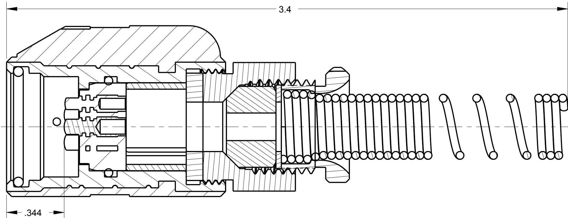
SECTION Z-Z
