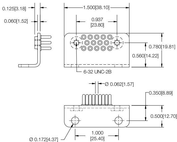
Grounding plate, part number: SK2484
