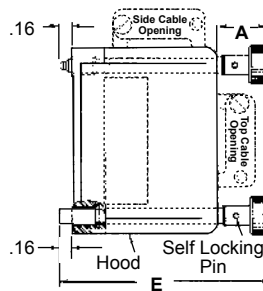
OR Mating connector half with Hood and turnable Long Jackscrews-with-Knobs. Code designation: JTC H, JTC H1
