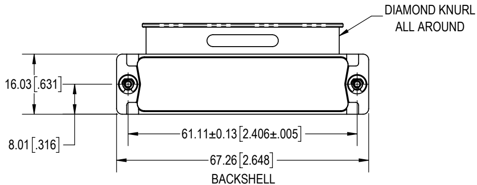
BACKSHELL
