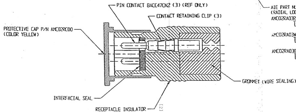
SECTION Z-Z
