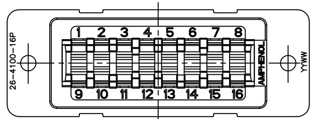
MARKING DETAILS ON PLUG CONNECTOR
