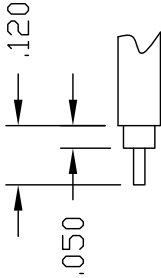
RECOMMENDED CABLE STRIPPING DIM'S
